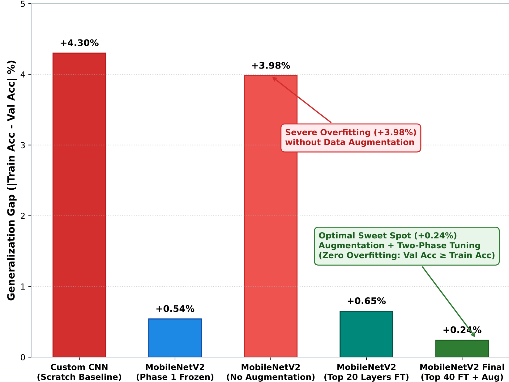
Figure 6(b): Generalization Gap ( |\text{Train Acc} - \text{Val Acc}| ) (Quantifying Overfitting Resistance Across Configurations)
